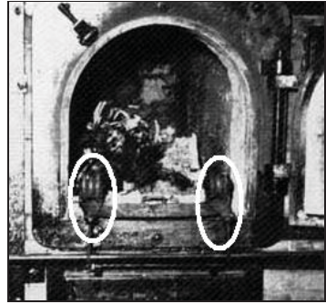
III. 1: Oven doors of the type used in the Auschwitz crematoria. Rollers to guide stretcher marked with white ellipses. 20
