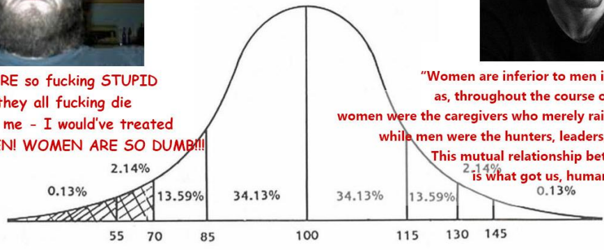
IQ bell curve
